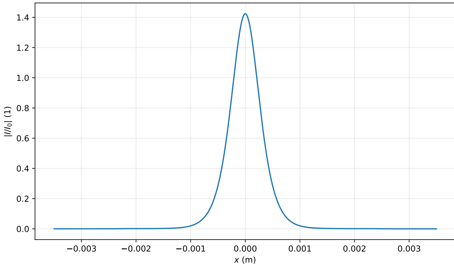
Intensity profile I(x, y = 0, z = 3.901m)/I_0 , P_{in}=0.9P_{cr} , artificial time
